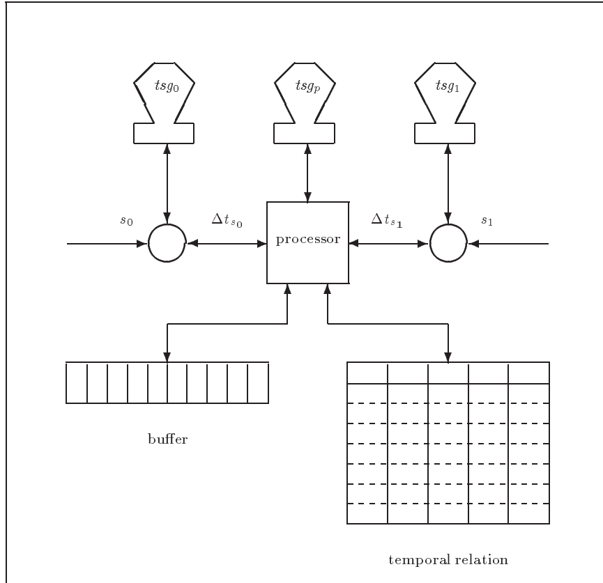
Figure 8: Buffering of Temporal Data.
