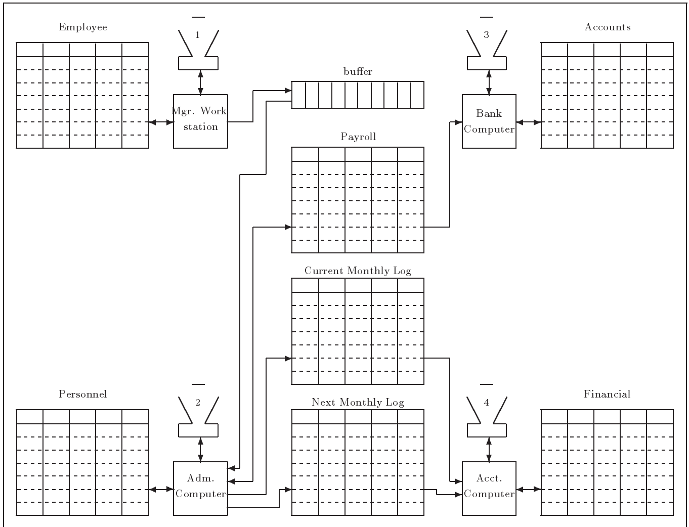
Figure 9: System Topology for the Extended Example
